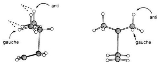
Figure 4. C_2 symmetrical ab initio UHF/3-21G transition structure for addition of the isopropyl radical to ethylene.
